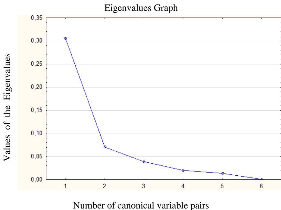
Figure 1. The chart of eigenvalues for canonical variables
